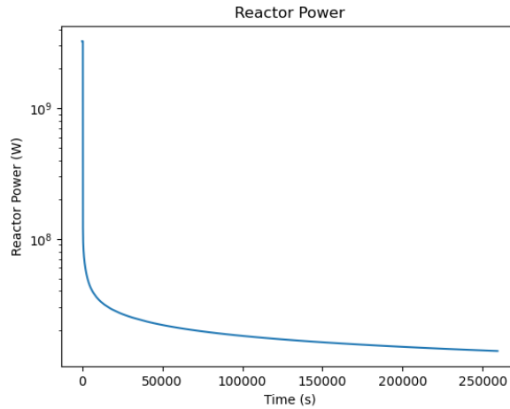
Figure 19: Core Power
